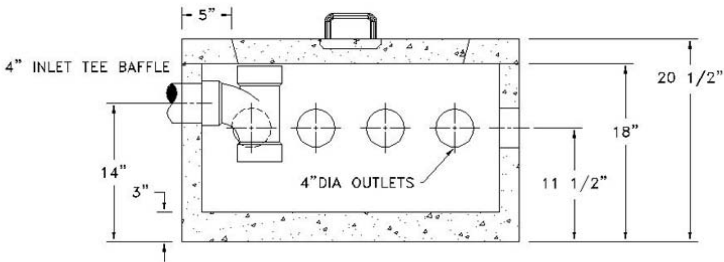
SECTION
